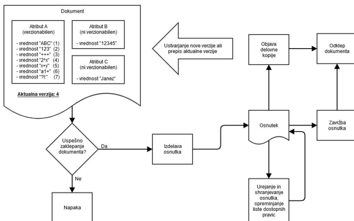
Image 33: Versioning process
