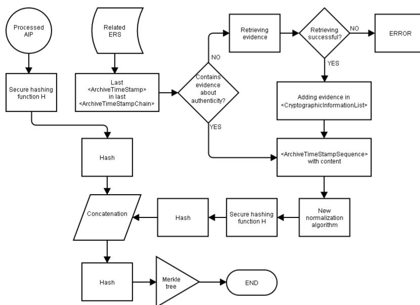
Image 22: Processing an AIP and its associated ERS
