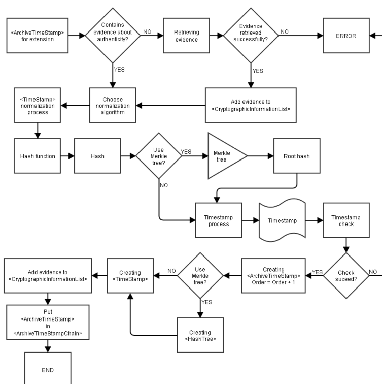
Image 21: Simple archive timestamp renewal
