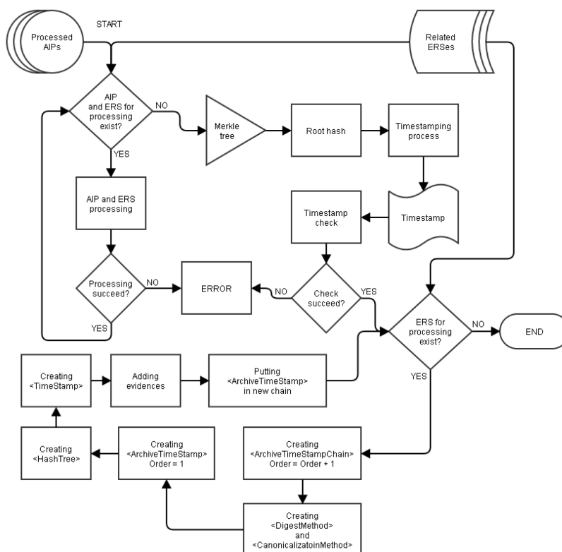
Image 23: Complex renewal with a Merkle tree
